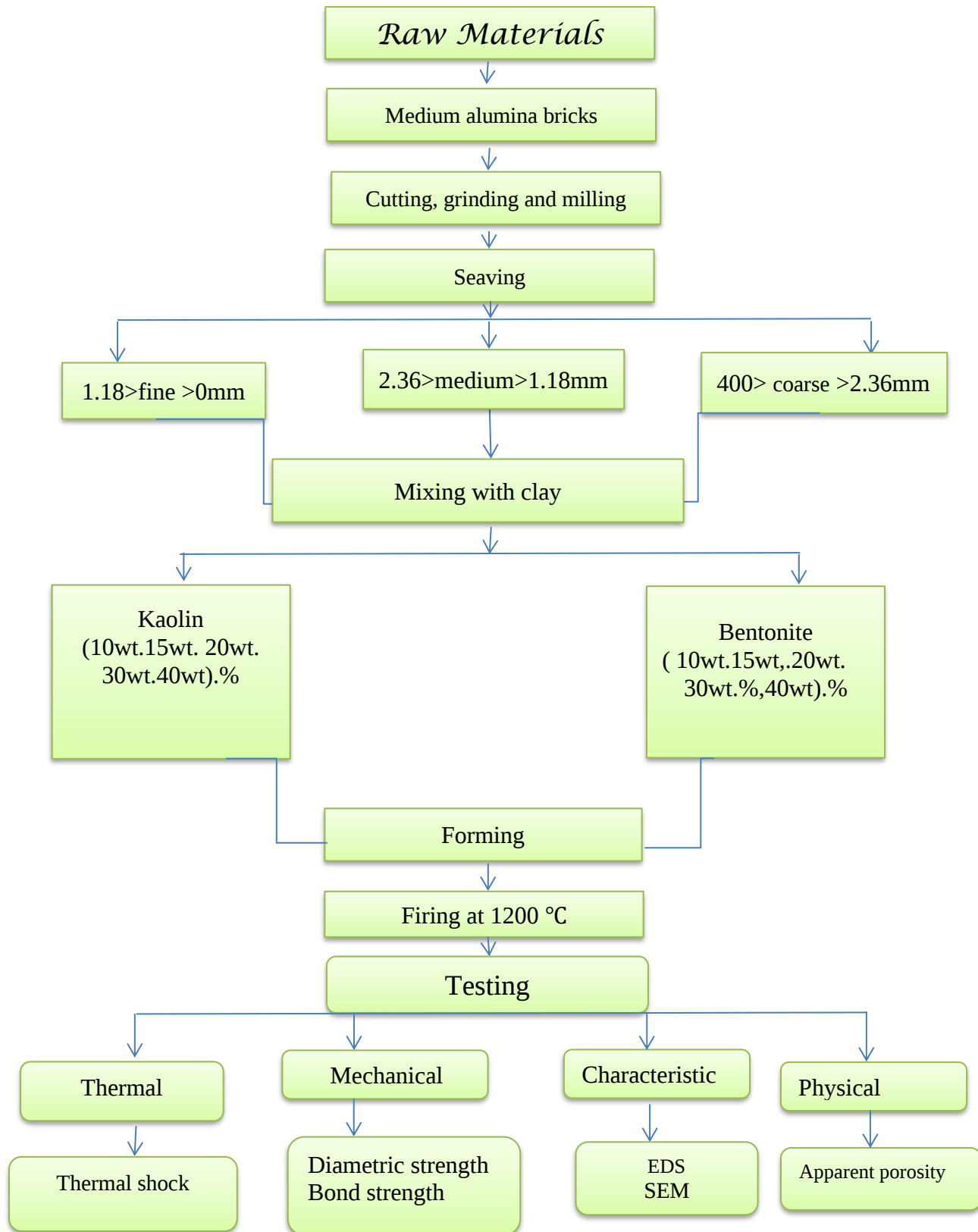
Figure 2: Chart of the experimental work.
