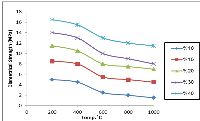
Figure 6: Diametrical Strength for kaolin mortar.
