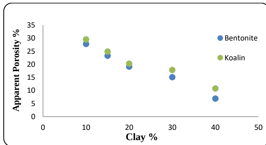
Figure 3: Apparent porosity for K-mortar and B-mortar.
