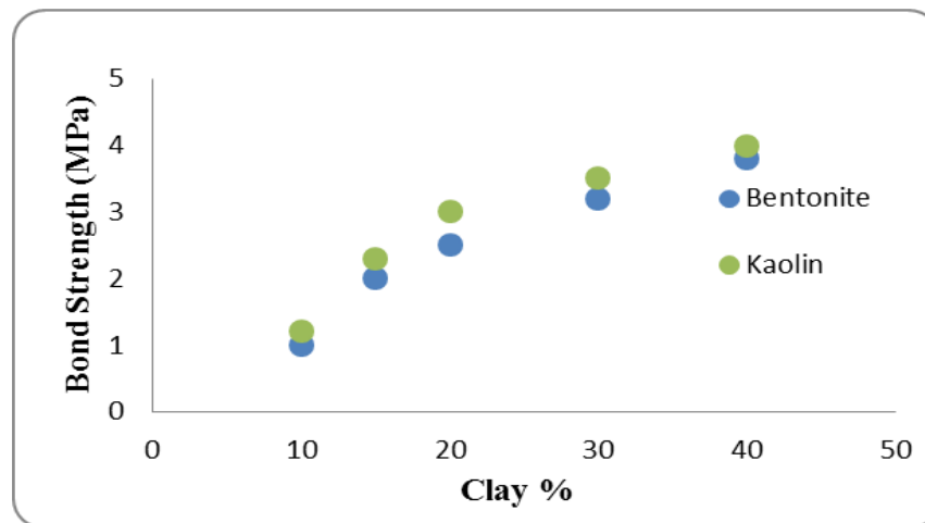
Figure 4: Bond strength for K-mortar and B-mortar.
