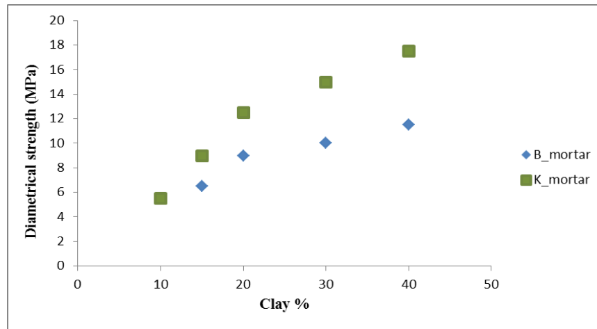
Figure 5: Diametric strength for K-mortar and B-mortar.
