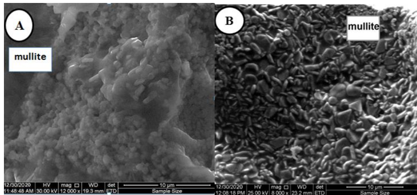
Figure 12: SEM images for prepared mortar specimen's surfaces (A) Bentonite Mortar (B) Kaolin Mortar.
