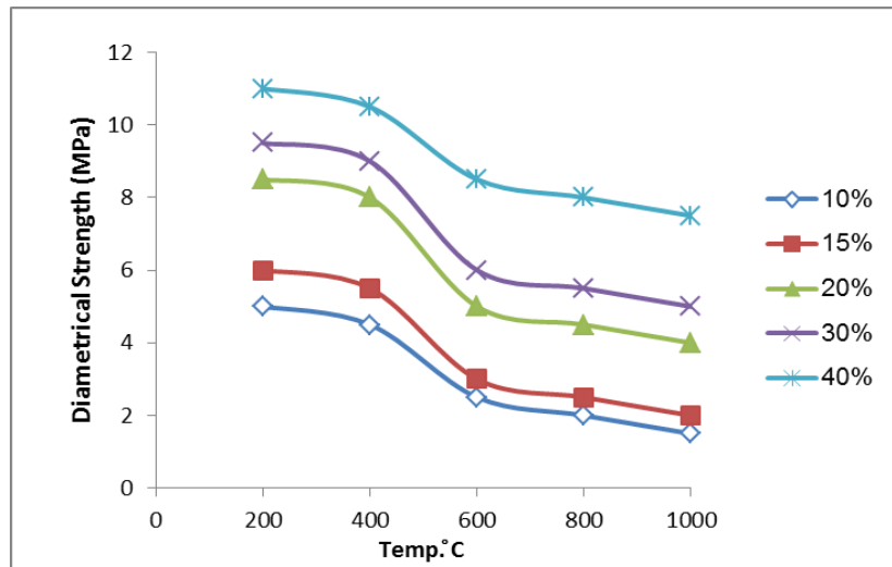
Figure 7: Diametrical Strength for bentonite mortar.
