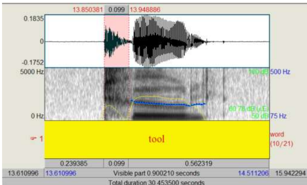
Figure (3): Wave Form of Initial [tʰ] with VOT Value 99ms of 'tool'.
