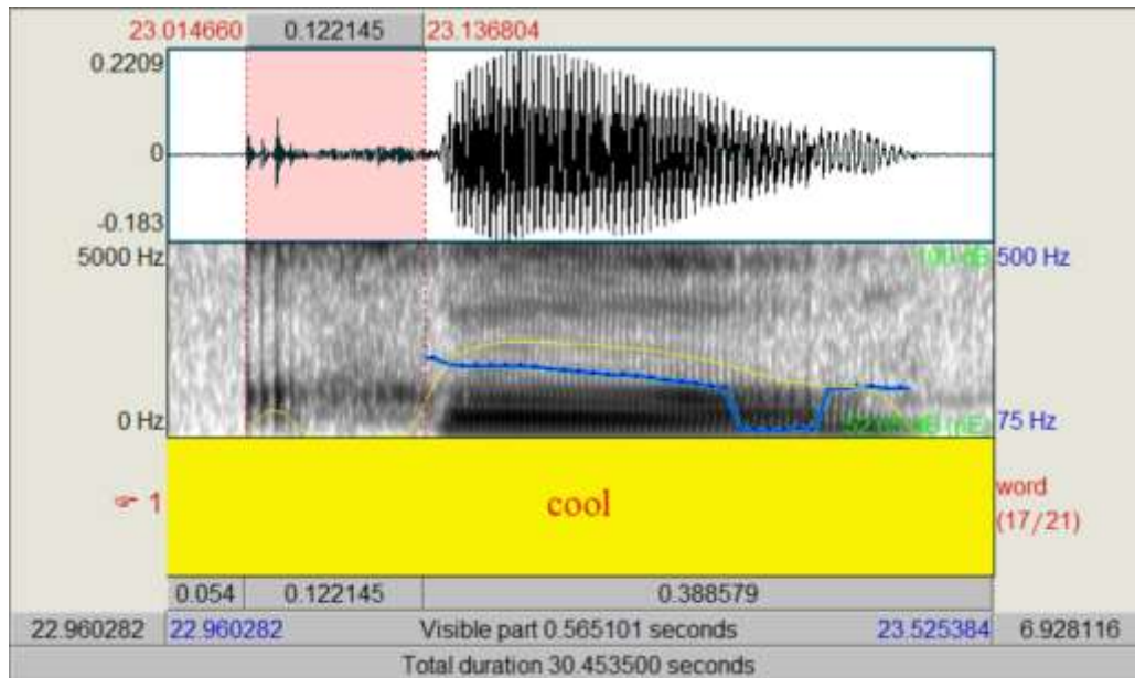
Figure (6): Wave Form of Initial [kʰ] with VOT Value 122 ms of 'cool'.
