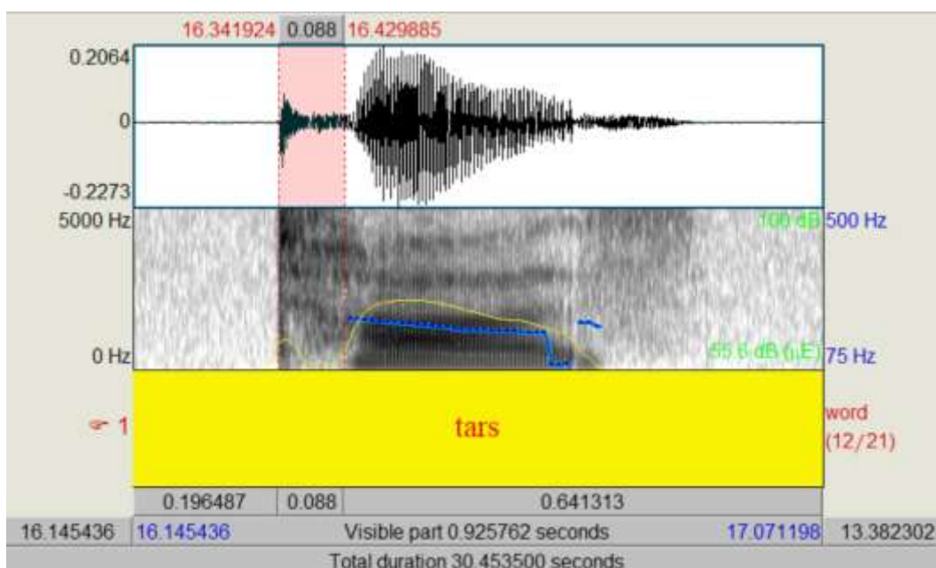
Figure (4): Wave Form of Initial [tʰ] with VOT Value 88 ms of 'tars'.
