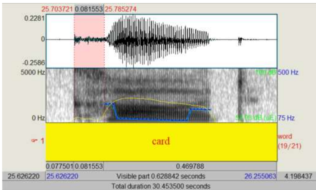
Figure (7): Wave Form of Initial [kʰ] with VOT Value 81 ms of 'card'.
