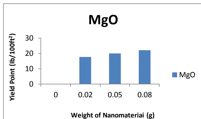
Figure 7: Effect of Nano-magnesium oxide Weight on Yield point of attapulgite water-based Mud.
