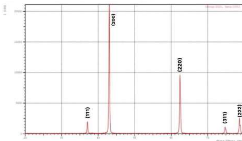
Figure 4: XRD Analysis of MgO nanoparticles
