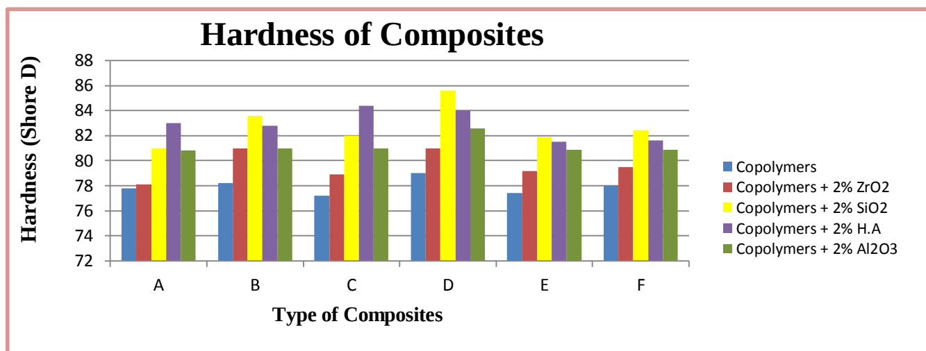
Figure 6: Hardness of prepared composite as a function of fillers type and the type of polymer blends for matrix material.
