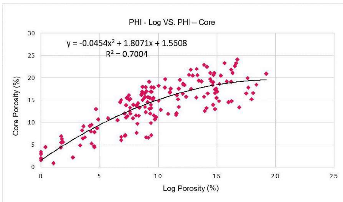
Fig. 6: The correlation between core-derived porosity and log-derived porosity of B-11 well.
