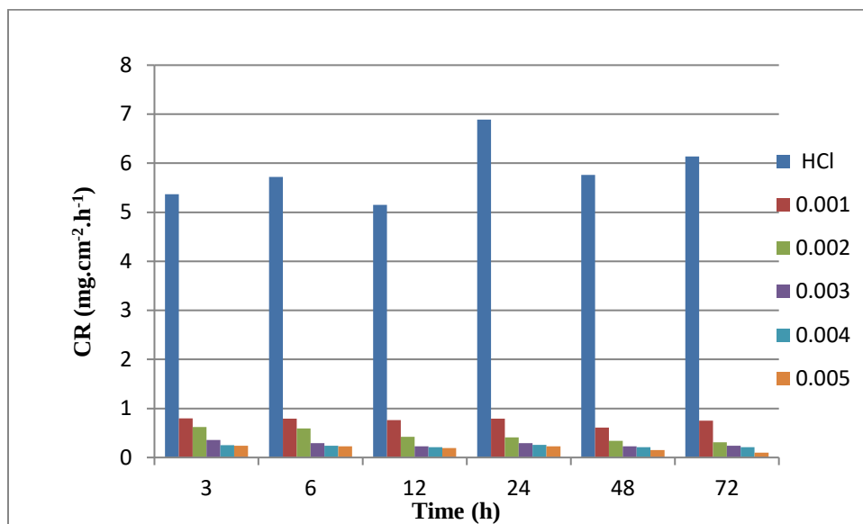
Figure 4: Corrosion rate for diverse immersion time at different concentrations of ABCP.
