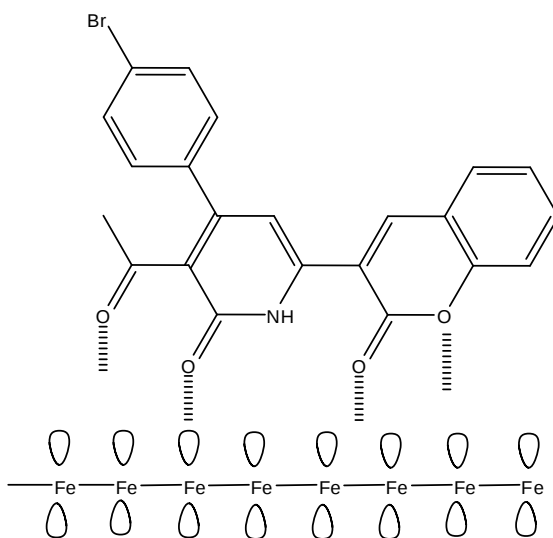
Figure 9: The suggested action on corrosion inhibitor of the ABCP molecule mechanism.
