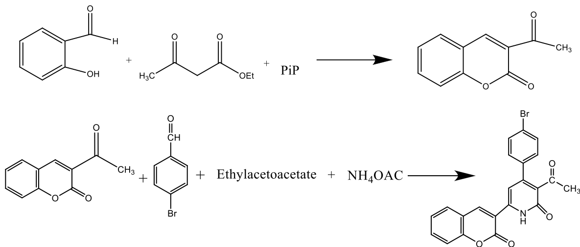
Figure 3. The reaction synthesis of ABCP.
