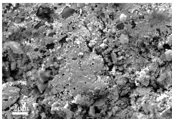
Figure 7: The SEM micrograph in the absence of the corrosion inhibitor for mild steel (ABCP).
