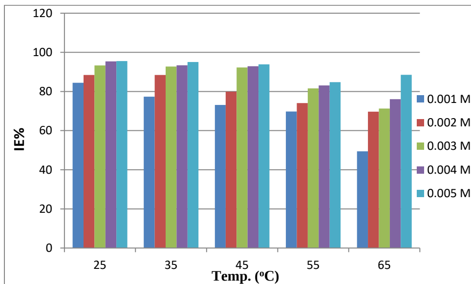
Figure 6: Inhibition Efficiency for different temperatures at varied ABCP concentrations.
