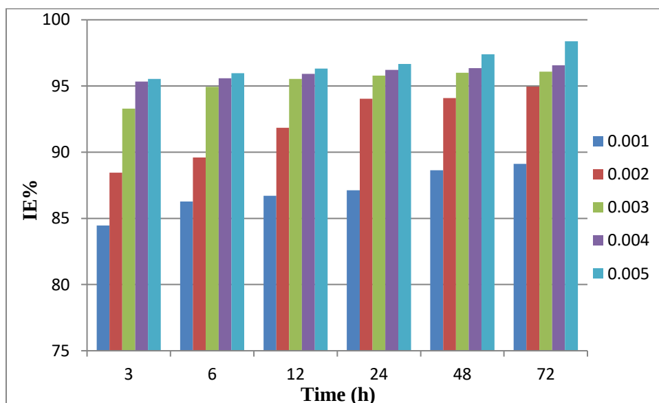
Figure 5: Inhibition Efficiency of different ABCP concentrations at different times of immersion.
