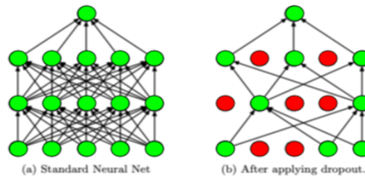
Fig. 5. Dropout Layer.
