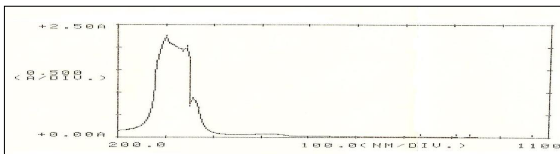
Fig.(3.a )The(UV - Vis) spectrum of [Co H_2L]_2
