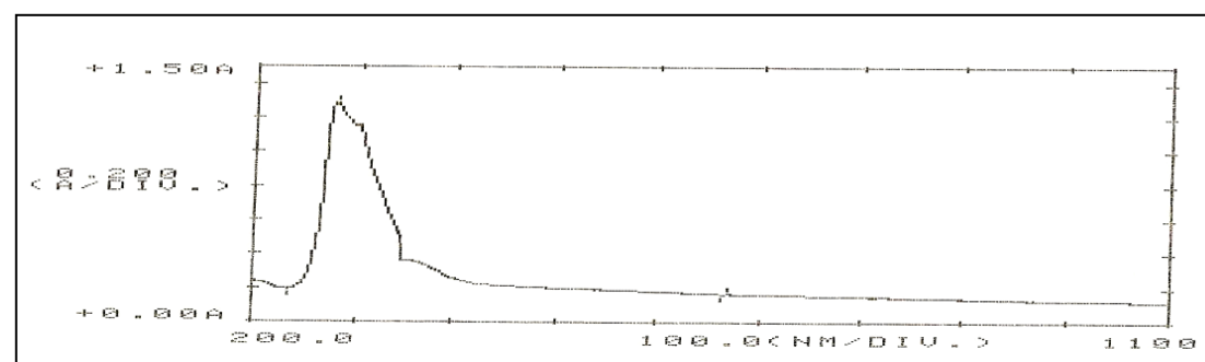
Fig.(3.a )The(UV - Vis) spectrum of [Co H_2L]_2
