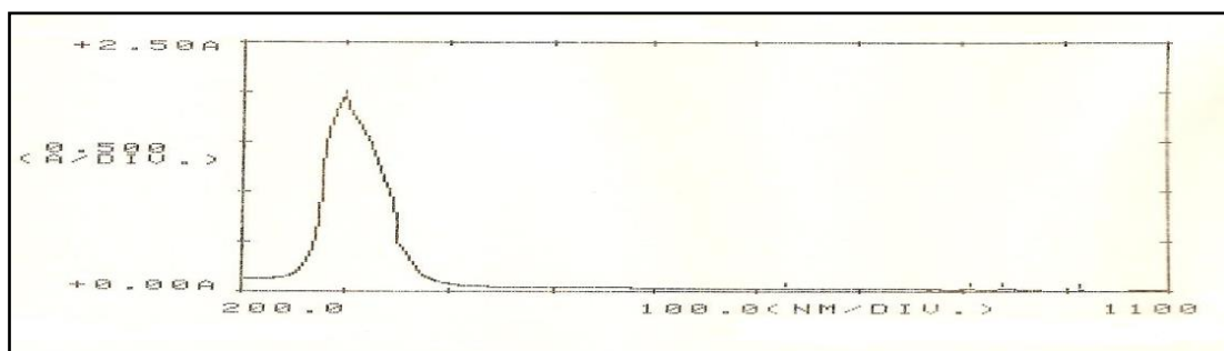
Fig.(3)The(UV - Vis) spectrum of ligand [H_3L]
