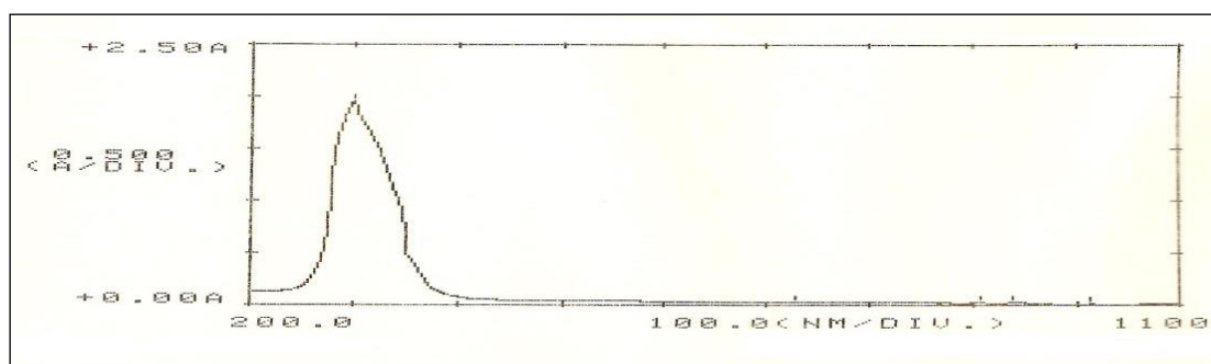
Fig.(3.C )The(UV - Vis) spectrum of [Zn H_2L]_2
