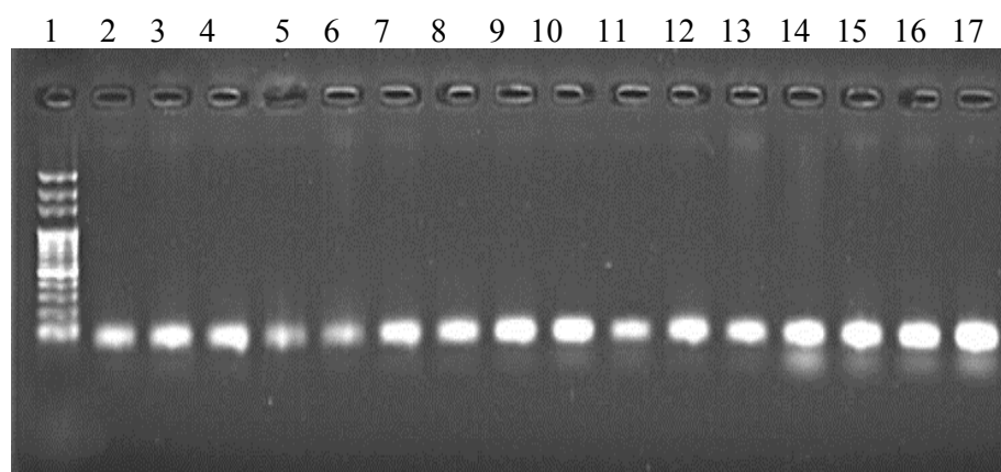
Figure 2: Electrophoresis pattern of PCR product forGhrelin gene, the amplification product was one band 90bp lane 2-9 PCR product for obese type 2 diabetes patients, lane 10-17 PCR products for control,1% agarose, 75v, 20 Am for 120 min.(10µl in each well).
