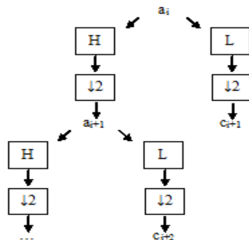
Figure (2) the high and low wavelet filters
