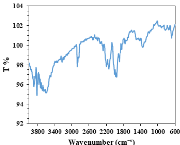
Figure 3: The FTIR analysis of biosynthesized AgNPs.
