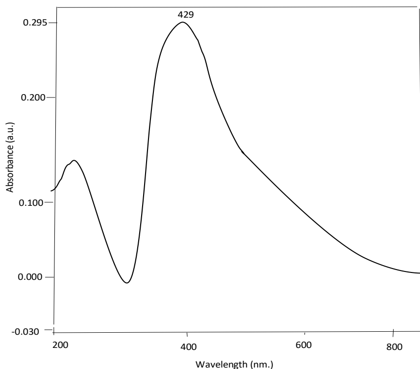
Figure 2: UV-Vis Analysis of Biosynthesized AgNPs.
