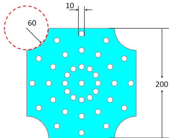
Figure 4: The proposed UC-PBG structure based SWCNT array
