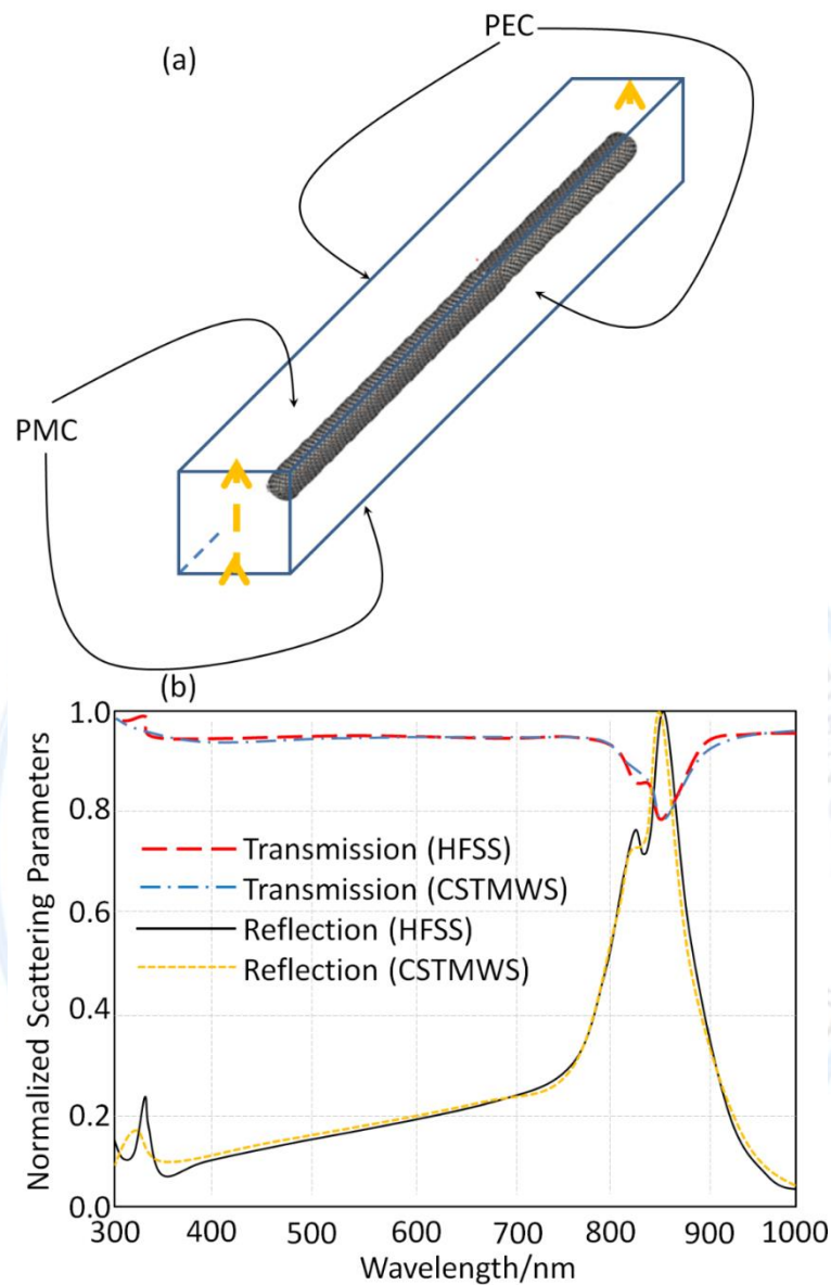
Figure 2: Vertical array of SWCNTs based HFSS and CSTMWS simulations; (a) The numerical setup, where, the yellow arrows are the excitation ports and (b) The obtained scattering parameters
