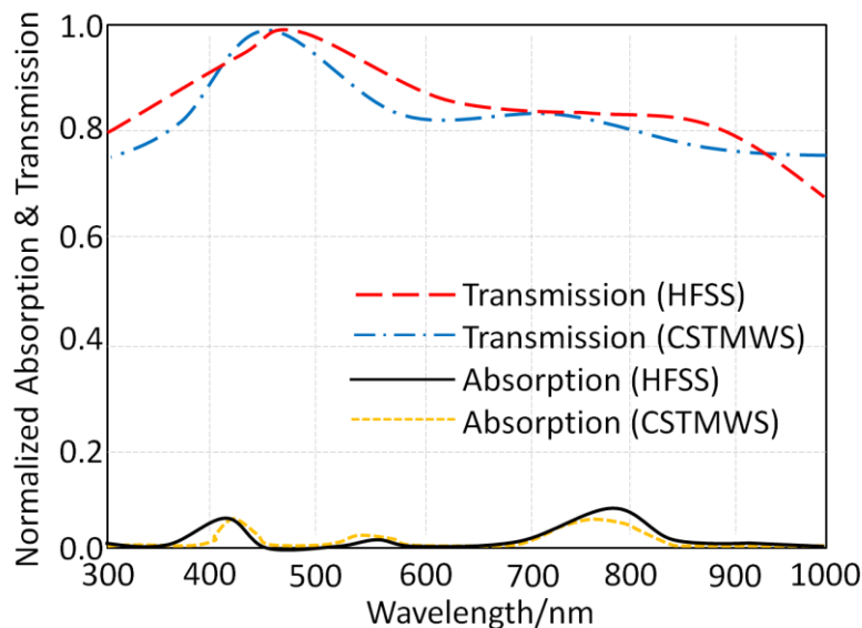
Figure 7: The normalized power of the absorption and transmission profiles of the proposed UC-PBG structure
