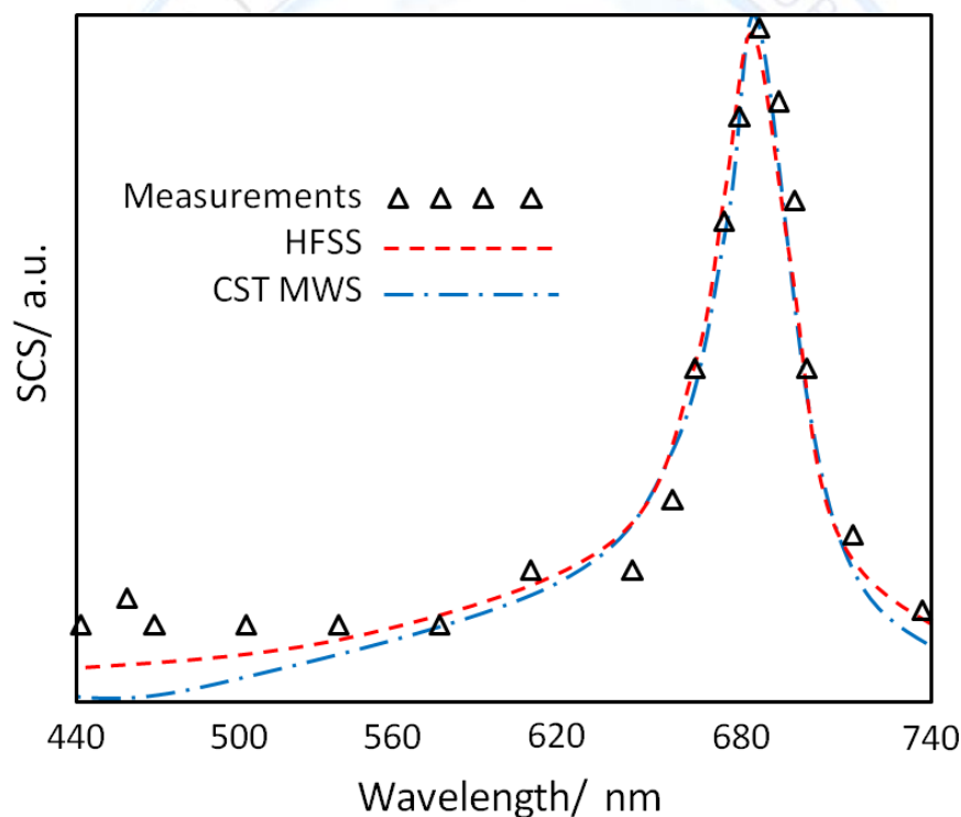
Figure 1: The numerical results of SCS verses measurements
