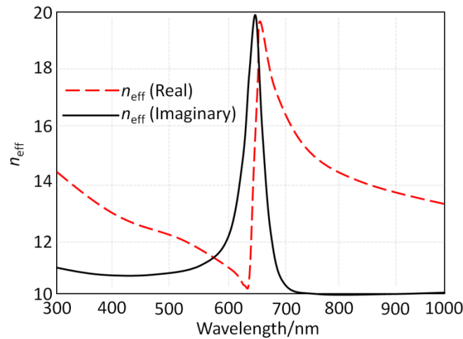
Figure 3: The retrieved n_{eff} of the vertical SWCNT array in terms of real and imaginary parts
