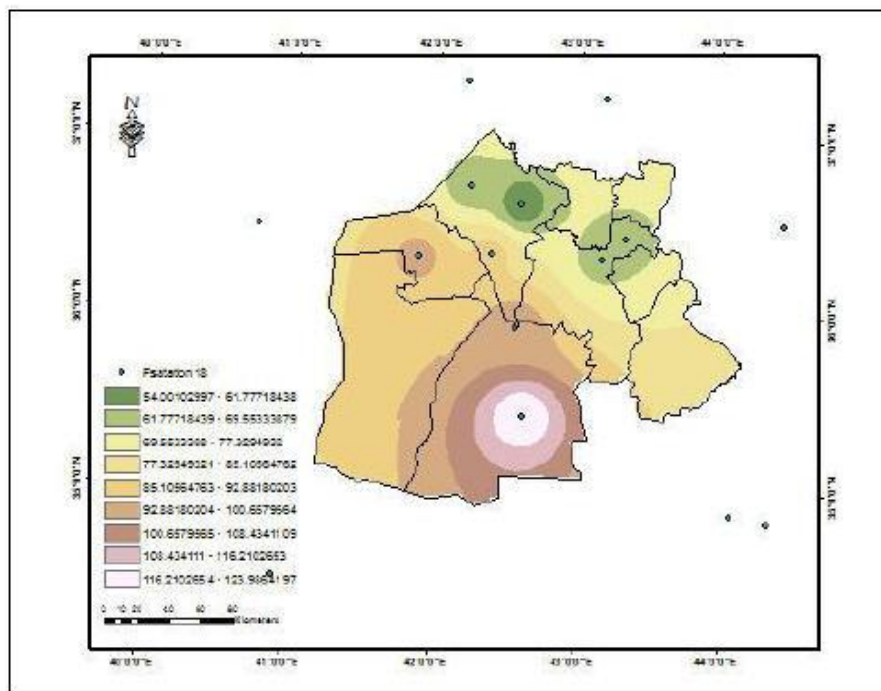
Figure 10: The predicted map of the power density for the selected stations
