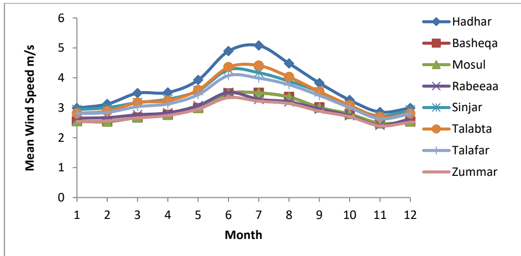
Figure 5: Monthly mean change of wind speeds in years (2000-2019) for chosen stations (in the height of 10 m).
