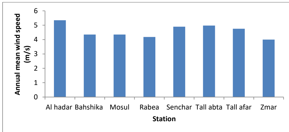
Figure 8: The annual mean of wind speed for chosen stations in the height of 50 m.
