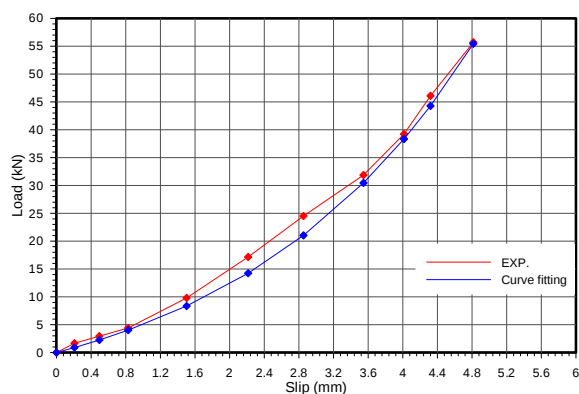
Fig. 8 Load-slip relationships, P2
