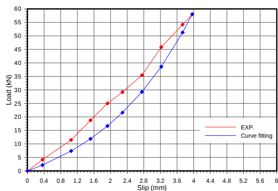
Fig. 9 Load-slip relationships, P3
