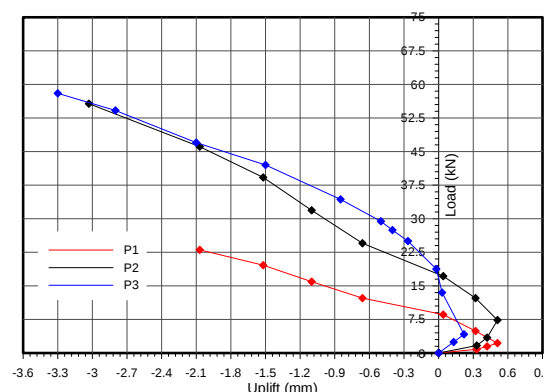
Fig. 6 Load-uplift relationships
