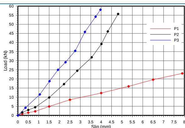
Fig. 5 Load-slip relationships
