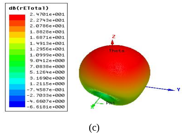
Figure. 3 Radiation co-cross polarizations patterns with and without metamaterial in a) E b) H-planes c) 3D radiation pattern
