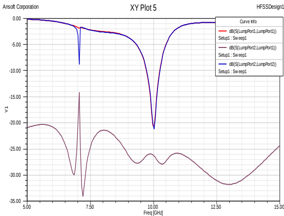
Figure. 8 Mutual coupling and reflection coefficients between two feeding ports with SRR metamaterial.
