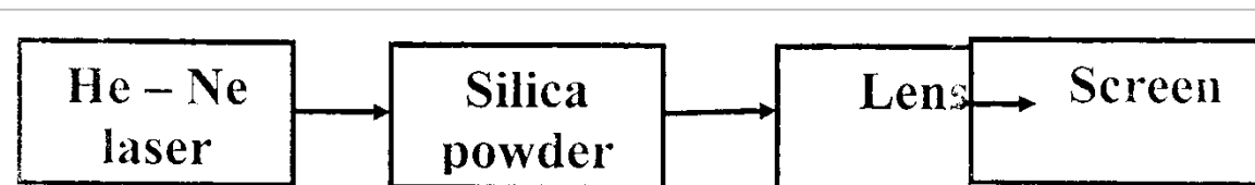
Fig(2) a block diagram of the measurement of diameter of silica
