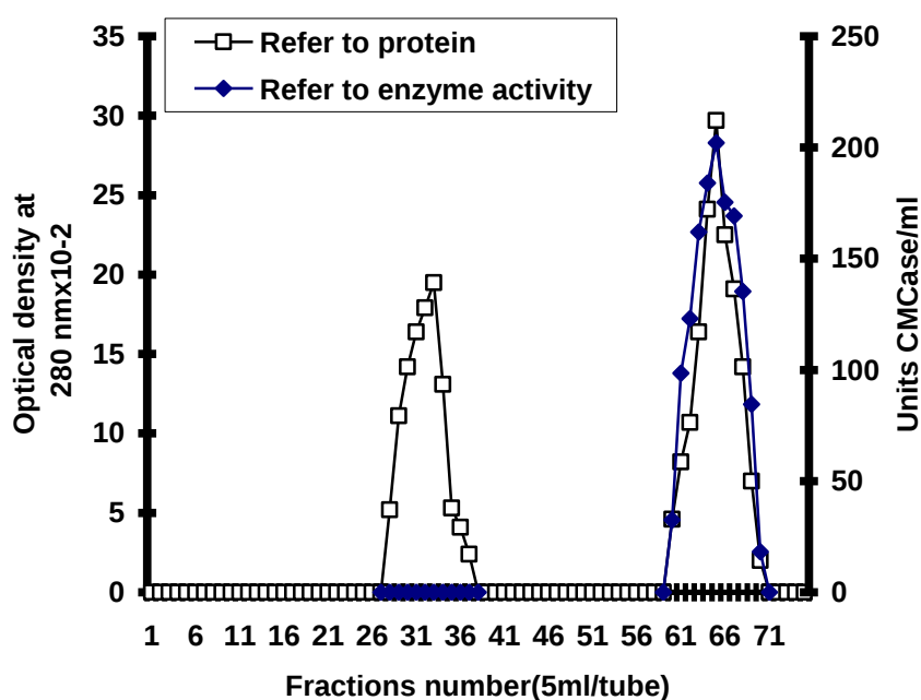
Figure (4): Sephadex G-150 chromatography of Enterobacter cloacae endoglucanase (CMCase)
