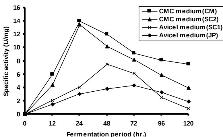
Figure (2): CMCase production in different culture media
