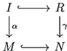
Diagram 10: N is sps-injective module.
