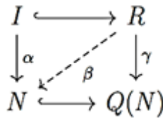
Diagram 9: N is sps-pure sub-module in Q(N) .
