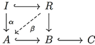
Diagram 8: A is sps-pure sub-module.
