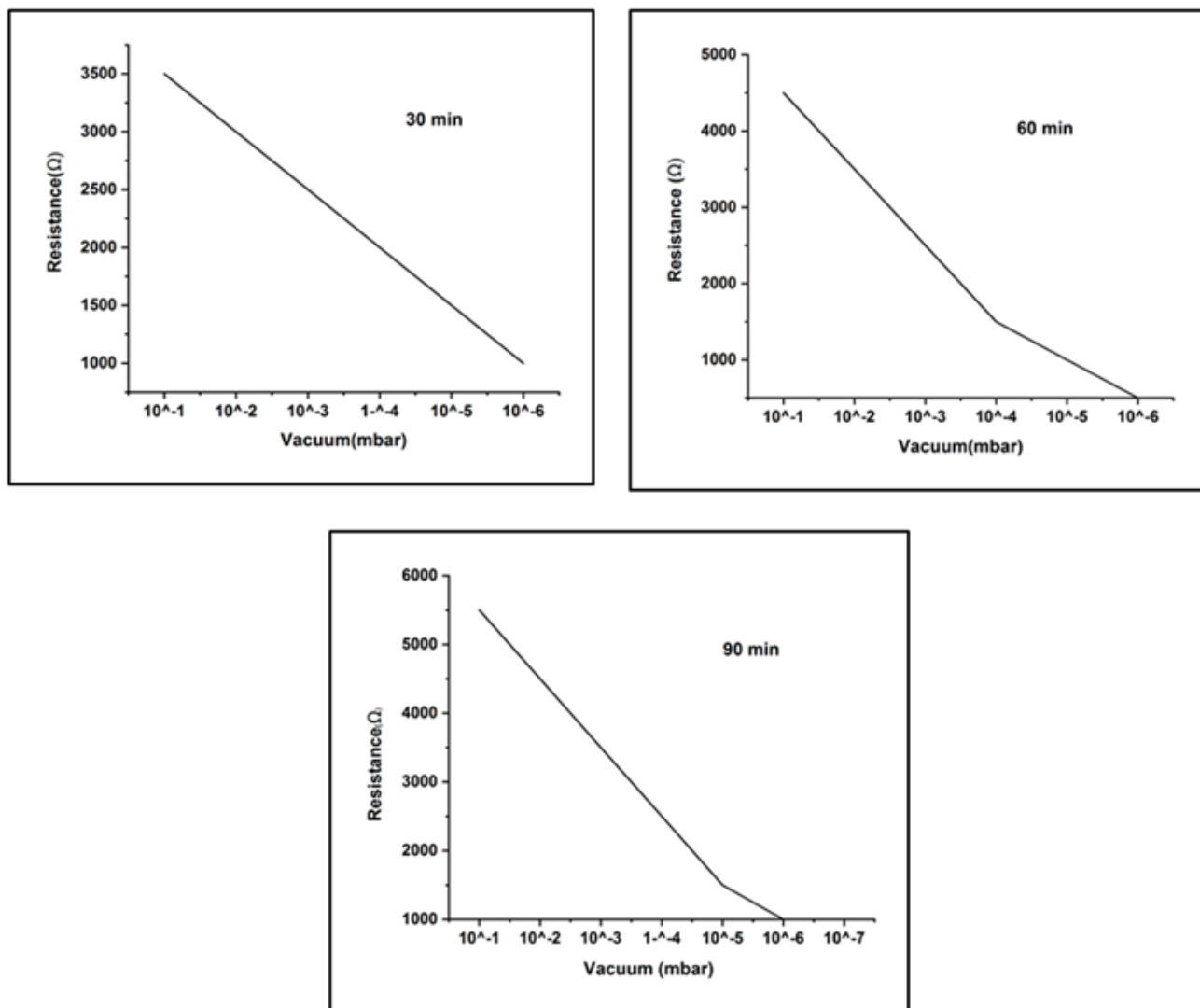
Figure 7: The relationship between the Electrical resistance of PSi and vacuum at etching time (30, 60, and 90) min at room temperature.
