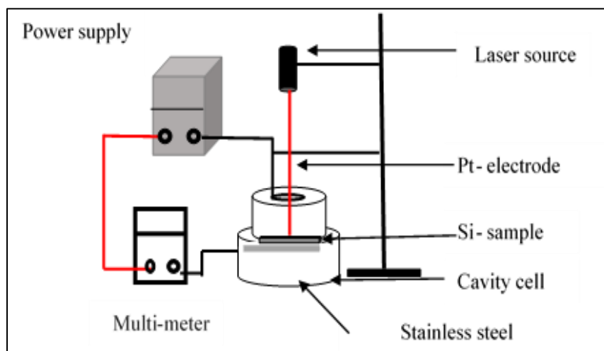
Figure 1: Schematic diagram of photo- electrochemical etching technique.
