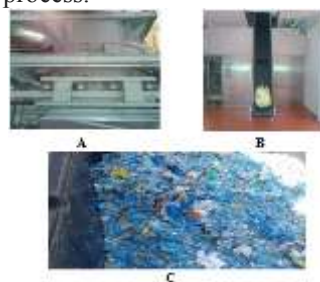
Figure (1): A: Shredder autoclave B: Transferring belt C: Medical wasted after being shredded and sterilized
