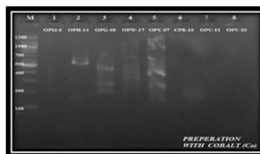
Fig. 4: Agarose gel electrophoresis of RAPD- PCR products. M: 100 bp DNA ladder, lines (1-8) positive result after treatment with CoFe 2 O 4 Nanoparticles.
