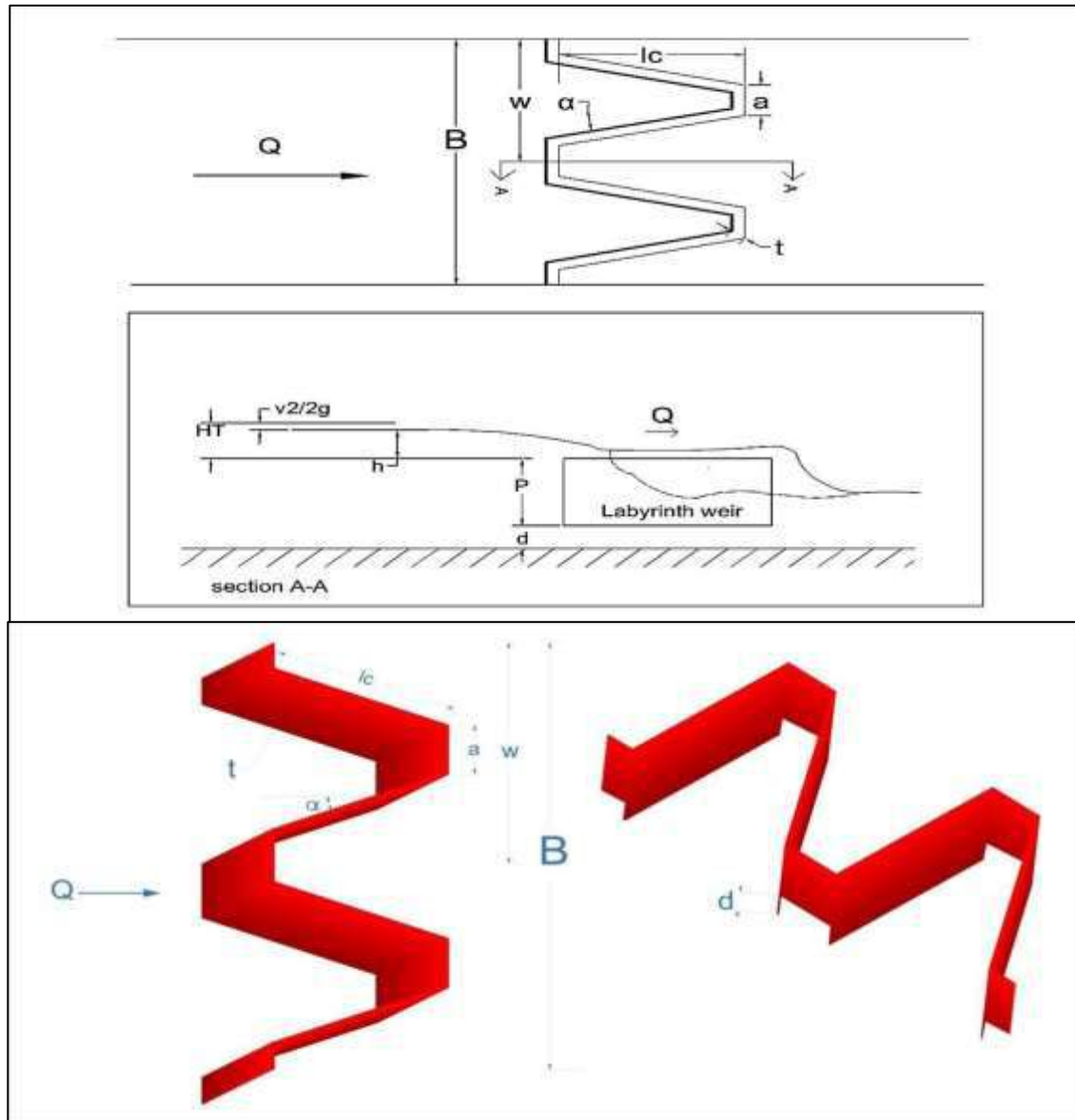
Fig. (1): Definition sketch of a top view, section, and schematic view with all dimensions of Combined Labyrinth weir-gate.
