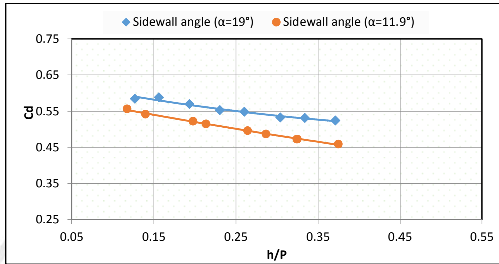
Fig. (8): Relation of the C_d and h/P for two models of combined labyrinth weirs-gate ( P=15\text{cm} ).
