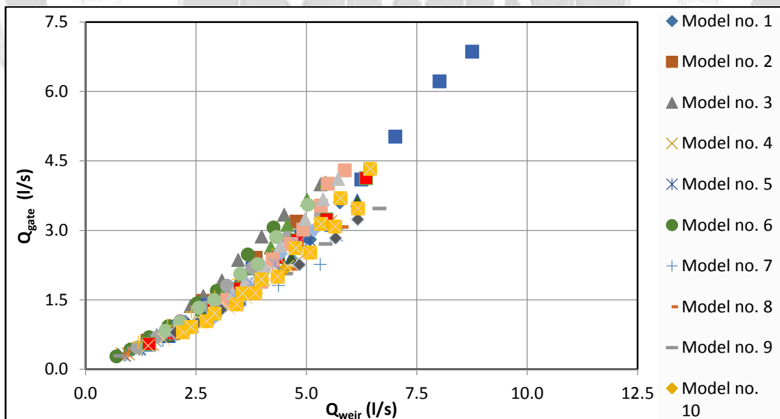
Fig. (10): Relation of the discharge of weir & gate for all models.
