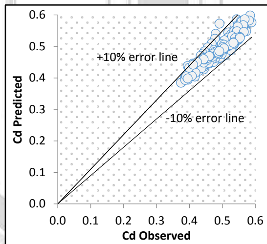
Fig. (9): Percentage error of C_d predicted for all models.
