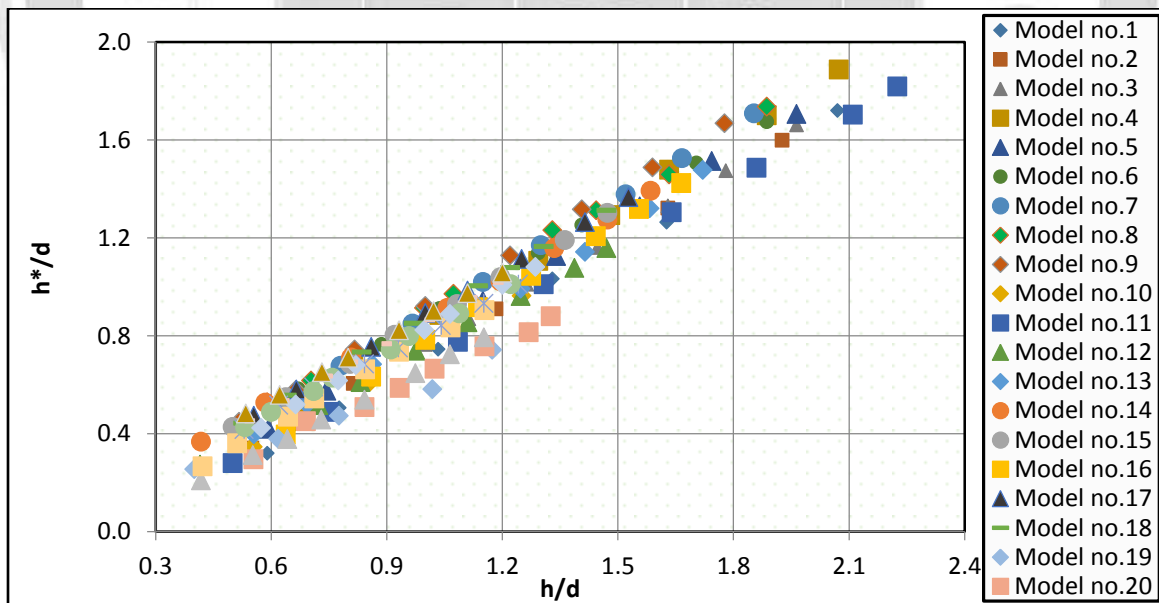
Fig. (11): Relation of h/d with h^*/d for the models.
