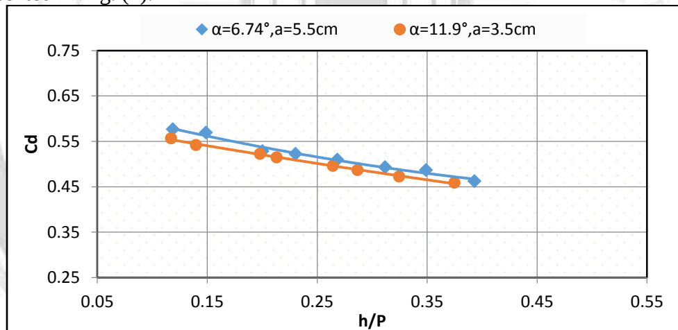
Fig. (7): Relation of the C_d and h/P for combined labyrinth weirs-gate ( P=15\text{cm} ).
