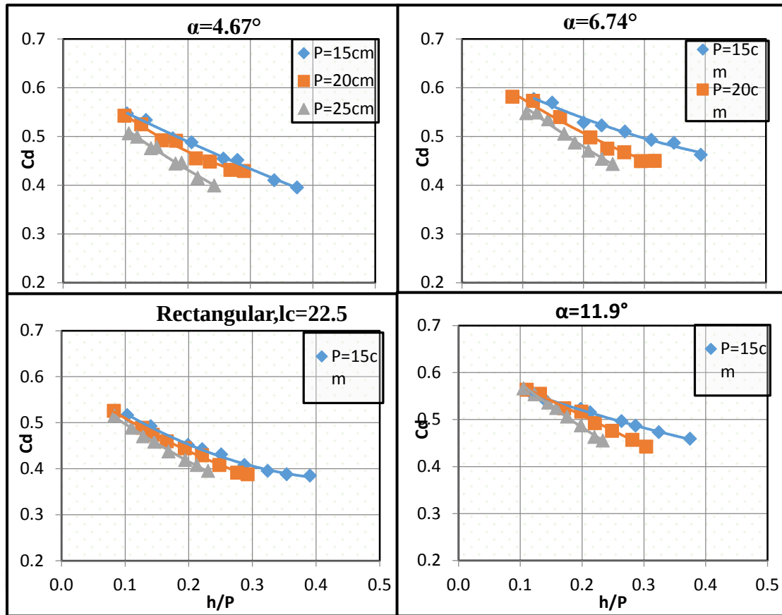
Fig. (3): Relation of the value of C_d and h/P for the combined labyrinth weirs.
