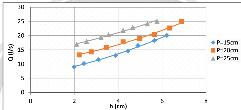
Fig. (2): Relation of Q and h for the combined labyrinth weirs.
