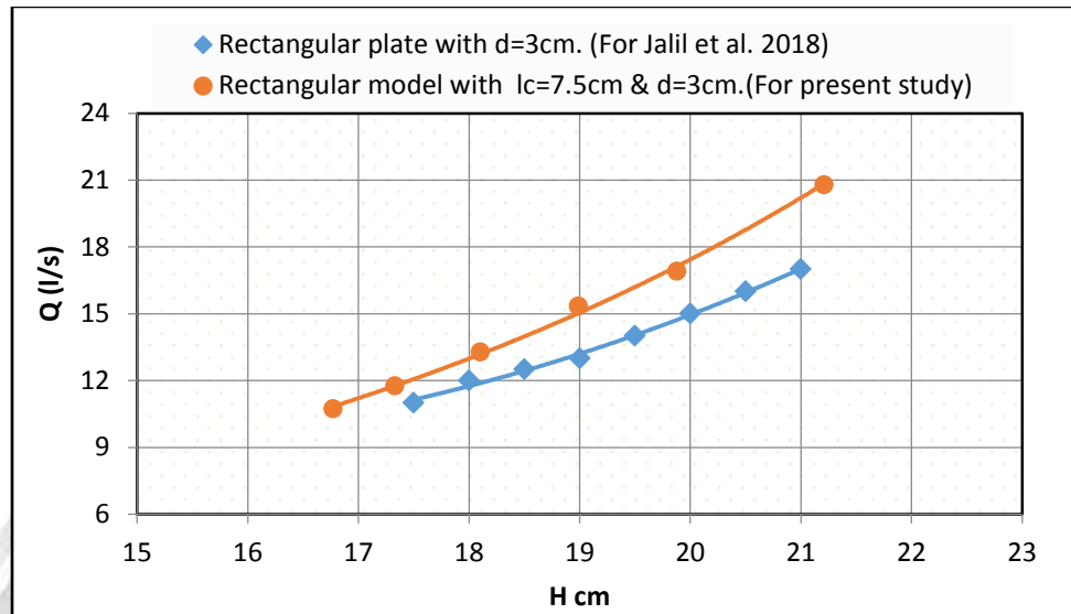
Fig. (6): Comparing the normal and Labyrinth weirs.
