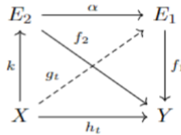
Fig. 2. M-Serre Fibration
