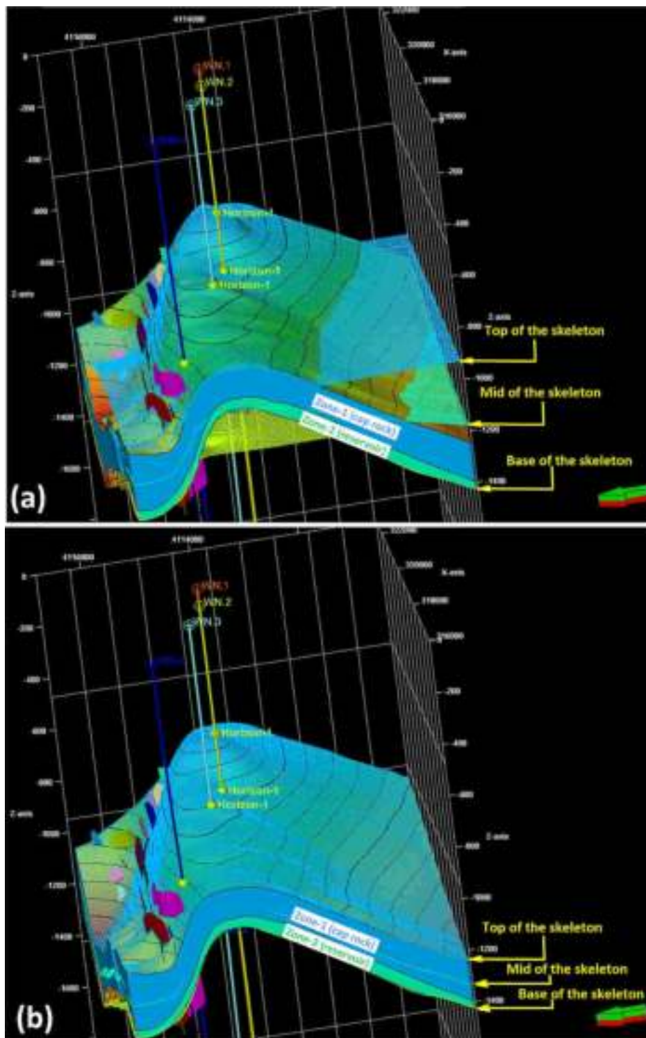
Fig.11. The grid skeleton (a) Fault-based modelling, the top of the skeleton and contours depth map of the Horizon-1 with the fault patch surfaces, and (b) Horizon-based modelling, the top of the skeleton and contours depth map of the Horizon-1 with the fault patch surfaces in their positions (arrows point northward).
