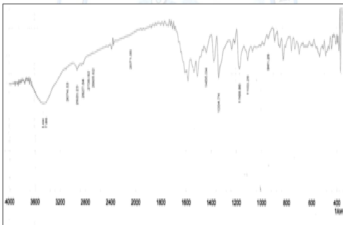
Figure No.(4): FT-IR spectra of compound (4)
