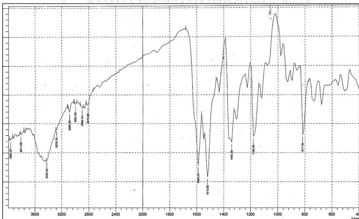
Figure No.(9): FT-IR spectra of compound (9)
