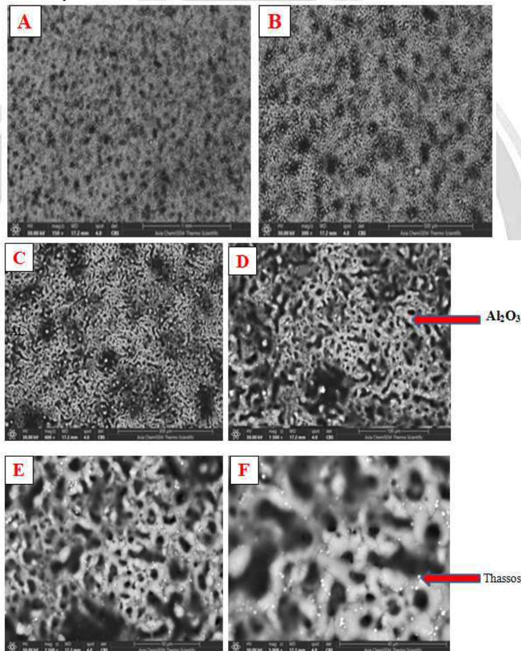
Figure 3: SEM Results for MC2.
