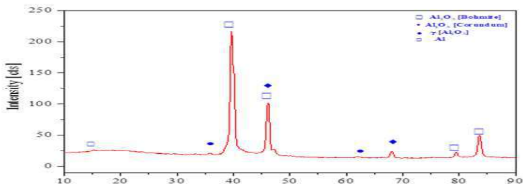
Figure 2: Results of XRD for MC2 Sample.
