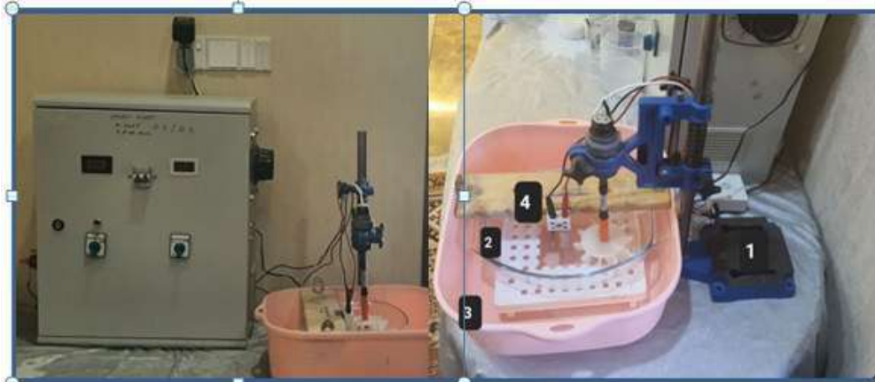
Figure 1: Images of the Coating Unit, (1) Mixer, (2) Coating Container, (3) Cooling Container, (4) Electrodes, (5) Thermometer.
