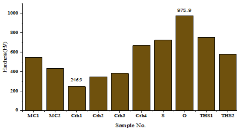
Figure 5: Hardness Results of Thassos Substrates.
