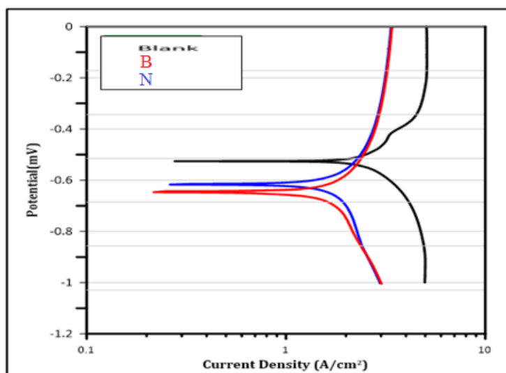
Fig . 6. Polarization curves for corrosion of blank HCl solution and N, and B.
