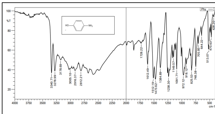
Fig.1. FT-IR spectra of compound [4-aminophenol]
