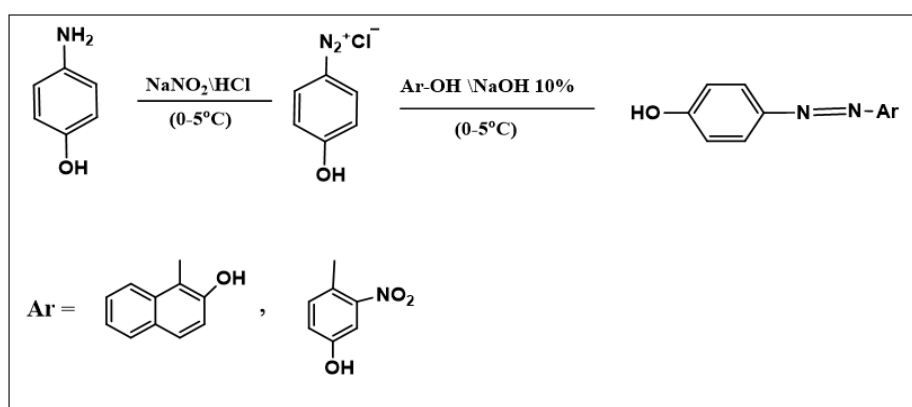
Scheme 1. Synthesis of compounds ( \beta - naphthol and 3-nitrophenol).
