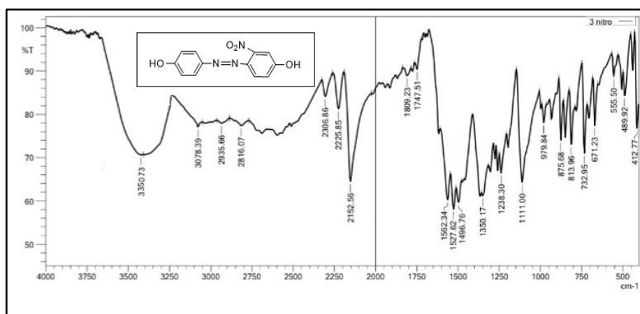
Fig .2. FT-IR spectra of compound (N).
