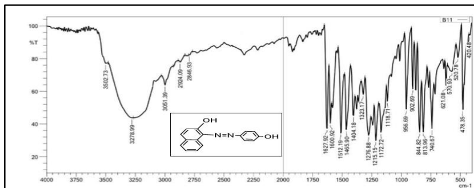
Fig.3. FT-IR spectra of compound(B).
