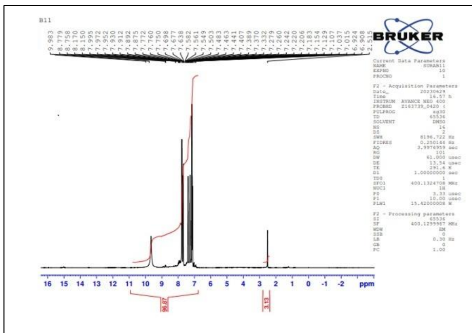
Fig.4. 1 H-NMR spectral (ppm) of compound(N).
