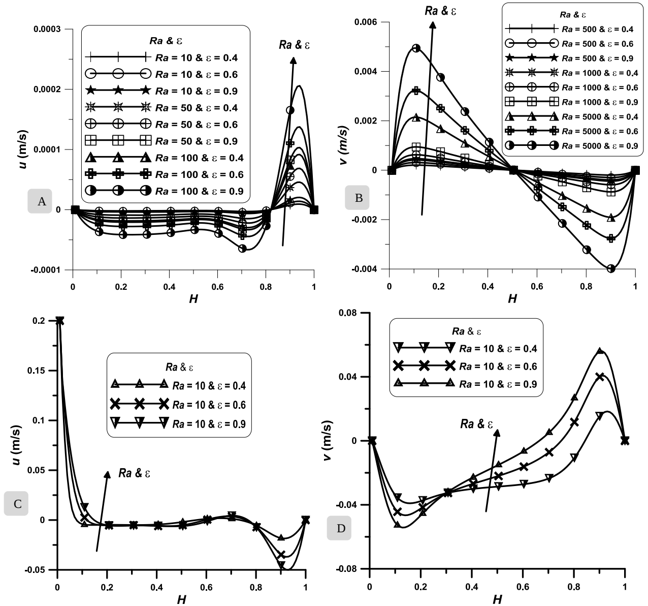
Figure 5 Velocities distributions at different Ra and \varepsilon .
