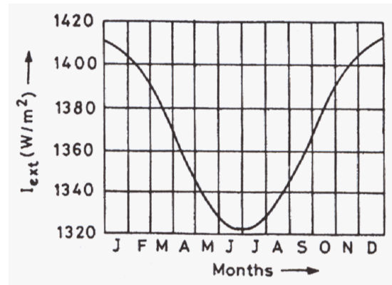
Figure 3 Variation of extraterrestrial solar radiation with time of the year
