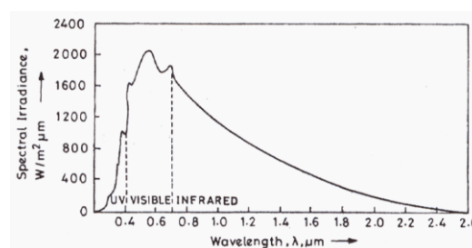
Figure 1 Spectral solar irradiance (Thekackara, M. P., 1977),
