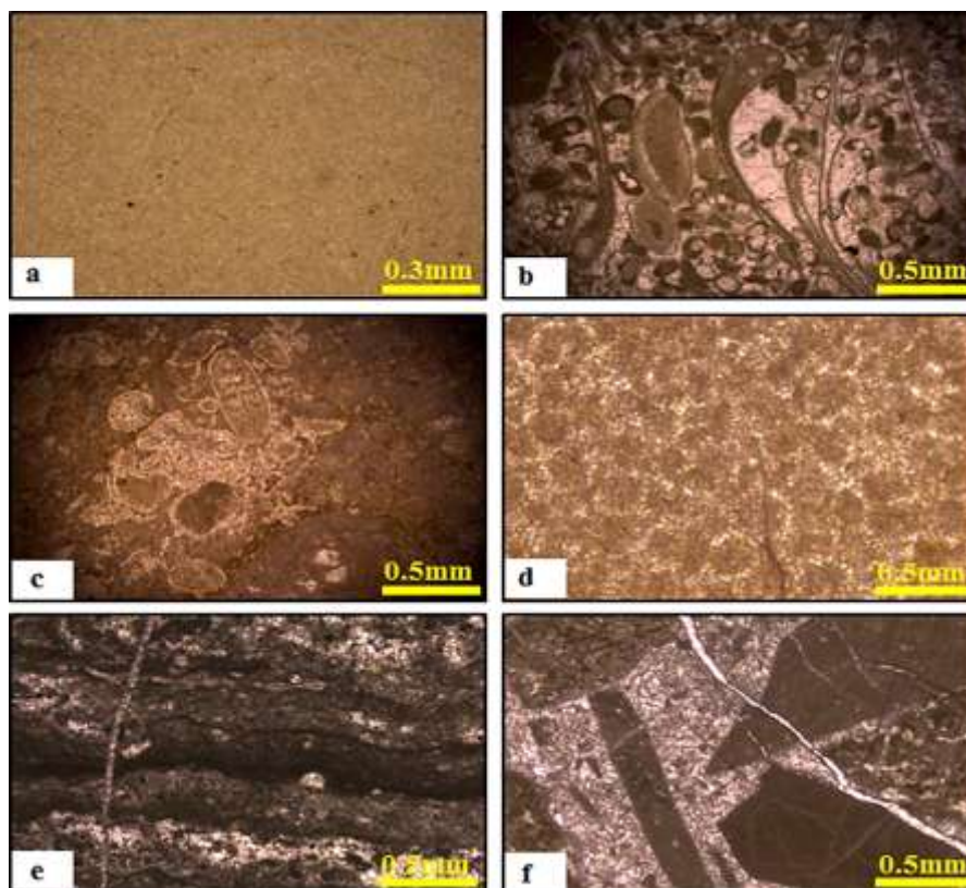
Fig. 9: Photomicrographs of Sarki Formation: (a) Dolomitized mudstone microfacies, which consist of microcrystalline dolomite and dolomicrite. WS. 1, X.N. (b) Ooidal bioclastic microfacies, ooids and valves of bivalve are the main component. WS. 31, P.P. (c) Bioclastic intraclastic packstone microfacies, major components are ostracod and intraclast in micrite groundmass. ZS. 2, P.P. (d) Ooidal grainstone microfacies, the main component are ooids and highly affected by dolomitization. ZS. 23, P.P. (e) Stromatolitic boundstone microfacies, the space mostly filled by different type of cements. WS. 34, P.P. (f) Recrystallized breccia, Most of the clasts are micritic and highly fractured, then filled by sparry calcite cement. ZS. 6, X.N., WS: Warte –Sarki, ZS: Zarwan-Sarki, P.P: Plane Polarized light, X.N: Crossed Nichols.
