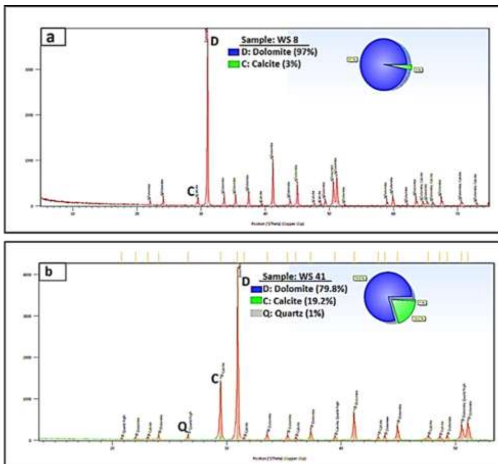
Fig. 6: XRD diffractograms for selected samples of the Sarki Formation.
