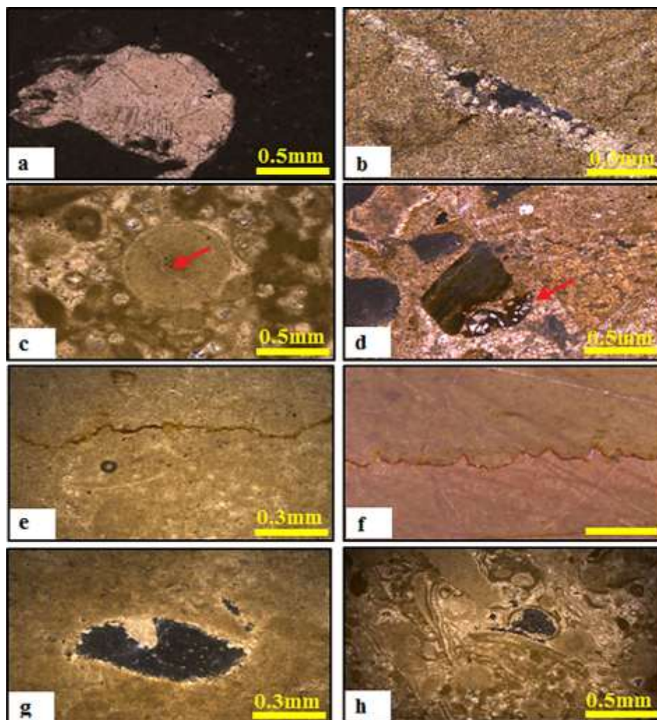
Fig. 8: Photomicrographs of Sarki Formation: (a) Blocky cement filling the mold of previously dissolved bioclast. WS. 38, P.P. (b) A fracture filled by granular cement, may indicate strong tectonic. WS. 14, X.N. (c) Breakage in a ooid grain, derived from compaction processes with silicification of quartz grains (arrow). (d) Deformation and plastic bending of intraclast showing wave appearance (arrow). ZS.6, P.P. (e) Sutured seam stylolite, irregular type with peaks of low amplitude, filled by bitumen SW. 27, X.N. (f) Sutured seam stylolite, irregular type with peaks of high amplitude (columnar stylolite). ZS. 7, P.P. (g) A moldic porosity formed by complete leaching and dissolution of ostracod grain. WS. 27, X.N. (h) Intraparticle porosity formed within ooid grain in ooidal bioclastic grainstone facies. WS. 42, X.N., WS: Warte –Sarki, ZS: Zarwan-Sarki, P.P: Plane Polarized light, X.N: Crossed Nichols.
