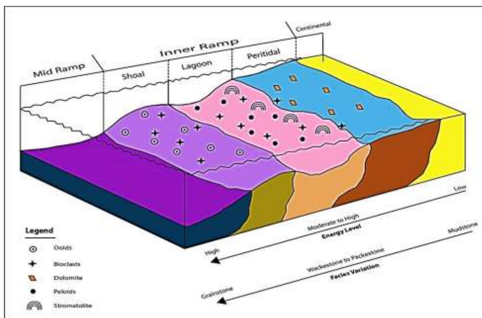
Fig. 10: Proposed depositional model for Lower Jurassic Sarki Formation.
