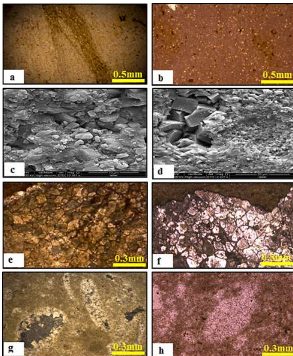
Fig. 7: Photomicrographs of Sarki Formation: (a) Iron oxide developed as fibrous shape in neomorphosed micrite matrix. WS. 17, X.N. (b) Fine crystalline planar-s (subhedral) dolomite. WS. 24, P.P. (c) SEM image of fine crystalline planar-s (subhedral) dolomite. WS. 41. (d) SEM image of fine to medium crystalline planar-e (euhedral) to planar-s (subhedral) dolomite. WS. 42. (e) Medium to coarse, planar-s (subhedral) to planar-e (euhedral) dolomites. ZS. 16, P.P. (f) Coarse crystalline, planar-s (subhedral) to nonplanar-a (anhedral) dolomites, pore between crystals filled by bitumen. ZS. 14, P.P. (g) Planar (euhedral) to planar (subhedral) void-filling dolomite cement. WS. 46, P.P. (h) Articulated ostracod filled by granular cement. WS. 46, P.P., WS: Warte –Sarki, ZS: Zarwan-Sarki, P.P: Plane Polarized light, X.N: Crossed Nichols.
