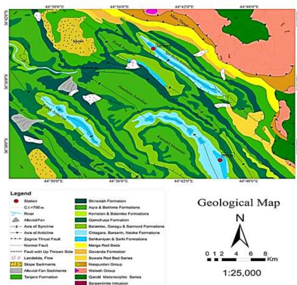
Fig. 2: Geological map of the studied sections, modified from [9].
