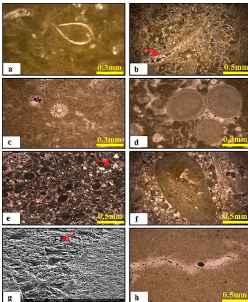
Fig. 5: Photomicrographs of Sarki Formation: (a) Articulated ostracod filled with micrite in bioclastic wackestone facies. WS. 31, P.P. (b) Inarticulate bivalves valve, curved shape, filled by drusy cement (arrow). WS. 42, P.P. (c) Spines of echinoid single crystal calcite, envelope in dolomitic matrix. WS. 27, P.P. (d) Non-skeleton grains spherical (ooids) filled by micrite (micrite envelope). WS. 42, P.P. (e) Peloids with quartz fragments affected by silicification (arrow) in peloidal packstone microfacies. WS. 45, X.N. (f) An intraclasts surrounding by ooids grain and fragment of bivalves affected by micritization. WS. 42, P.P. (g) SEM image showing detrital quartz grains (arrow). WS.34. (h) Small cubic pyrite formed in vein of groundmass micritic matrix. WS. 40, P.P., WS: Warte –Sarki, ZS: Zarwan-Sarki, P.P: Plane Polarized light, X.N: Crossed Nichols.
