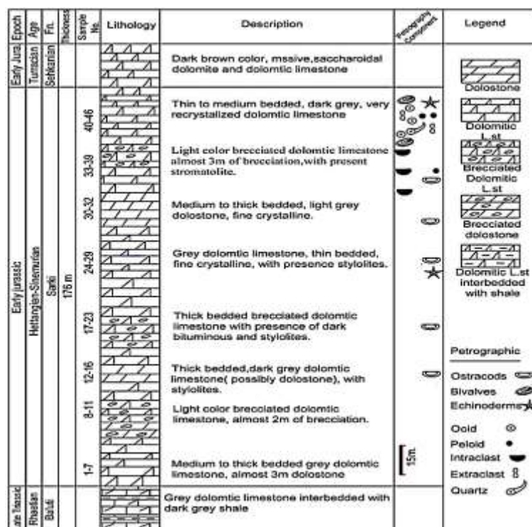
Fig. 3: Columnar section of Sarki Formation in the Warte section, Northeastern Iraq.
