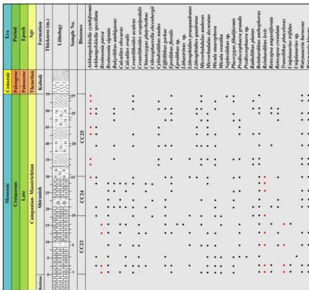
Fig.6: Calcareous nannofossils range chart for the Shiranish Formation from the studied area.
