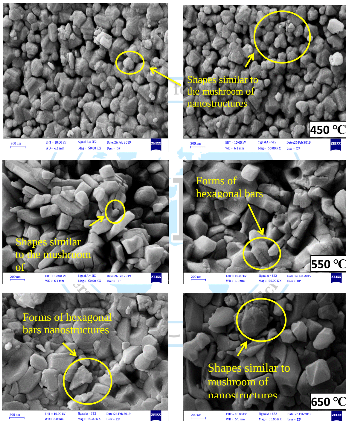
Figure 2: FESEM images of the compounds ( \text{MoO}_3 / \text{NiAl}_2\text{O}_4 ) prepared and coated with different temperatures
