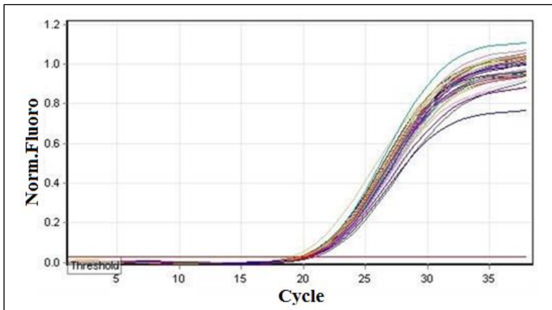
Figure 1: Amplification plots of a miR-122a gene by RT-qPCR.
