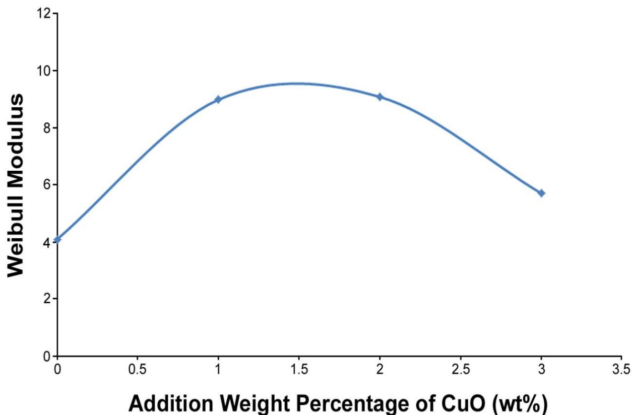
Figure 7: The relationship between Weibull modulus and addition weight percentage of CuO.
