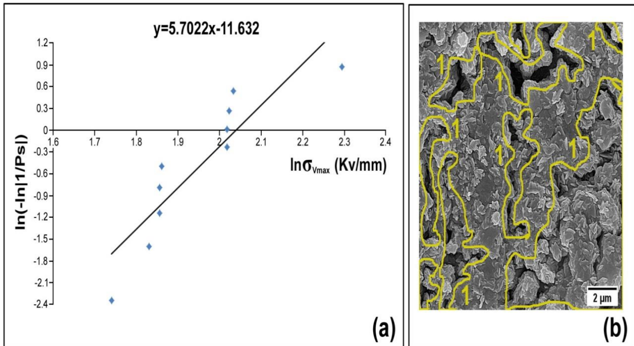
Figure 4: (a) Weibull modulus determination for LC3S as homogeneity indicator. (b) FESEM image for LC3S microstructure 2 \mu\text{m} .
