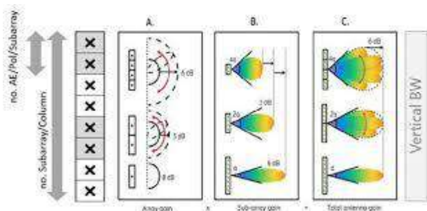
Fig .13: beamforming steering
