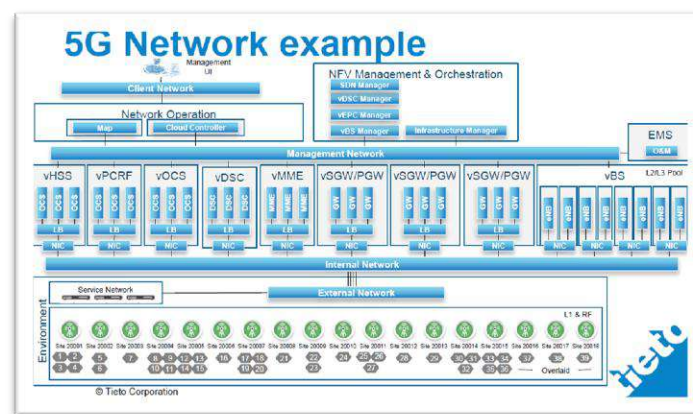
Fig .24: example of 5G network virtualization
