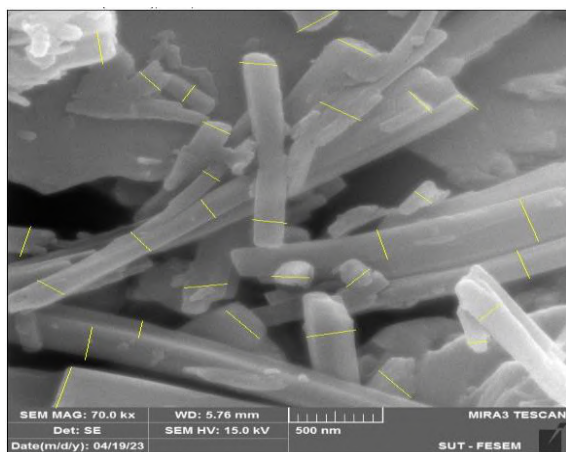
Fig. 8: SEM image of the complex [Hg_2(CHB)_2\mu-(dppe)Cl_2]Cl_2 at 500nm, and the particle sizes and Gaussian Fit curve for the complex [Hg_2(CHB)_2\mu-(dppe)Cl_2]Cl_2 at 500nm
