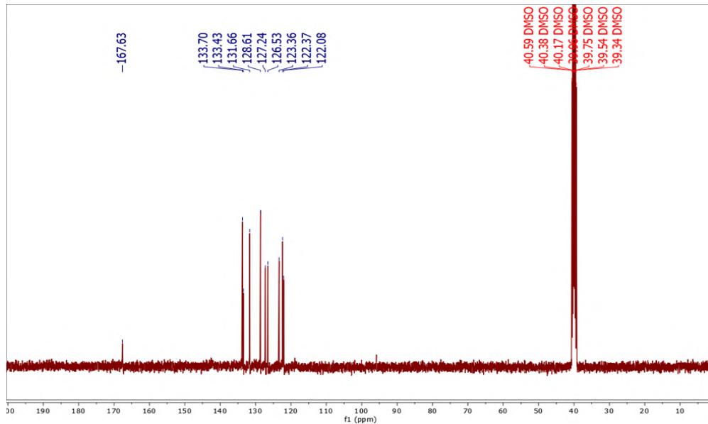
Fig. 2: ^{13}\text{C-NMR} spectrum of [CHB]
