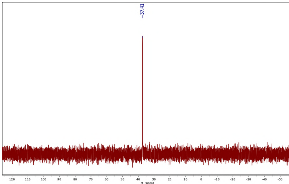
Fig. 6: ^{31}\text{P}\{-^1\text{H}\} -NMR spectrum of [\text{Hg}_2(\text{CHB})_2(\mu\text{-dppe})\text{Cl}_2]\text{Cl}_2
