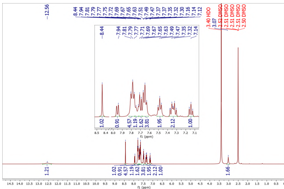
Fig. 5: H-NMR spectrum of [\text{Hg}_2(\text{CHB})_2(\mu\text{-dppe})\text{Cl}_2]\text{Cl}_2
