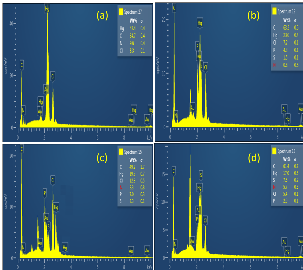
Fig. 11: Elemental structure of the complexes: (a) [\text{Hg}(\text{CHB})_2\text{Cl}_2] , (b) [\text{Hg}_2(\text{CHB})_2\mu\text{-(dppm)}_2]\text{Cl}_4 , (c) [\text{Hg}_2(\text{CHB})_2\mu\text{-(dppe)}\text{Cl}_2]\text{Cl}_2 , (d) [\text{Hg}_2(\text{CHB})_2\mu\text{-(dppp)}\text{Cl}_2]\text{Cl}_2
