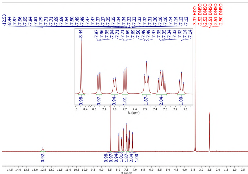
Fig. 1: ^1\text{H-NMR} spectrum of the ligand [CHB]
