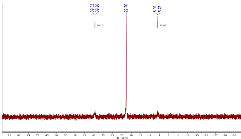
Fig. 4: 31 P-{ 1 H}-NMR spectrum of [Hg 2 (CHB) 2 (μ-dppm) 2 ]Cl 4
