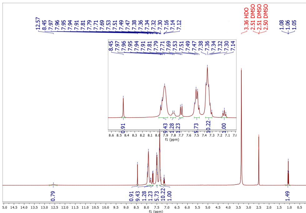
Fig. 3: 1 H-NMR spectrum of [Hg 2 (CHB) 2 (μ-dppm) 2 ]Cl 4
