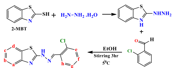
Scheme 1: Ligand preparation equation
