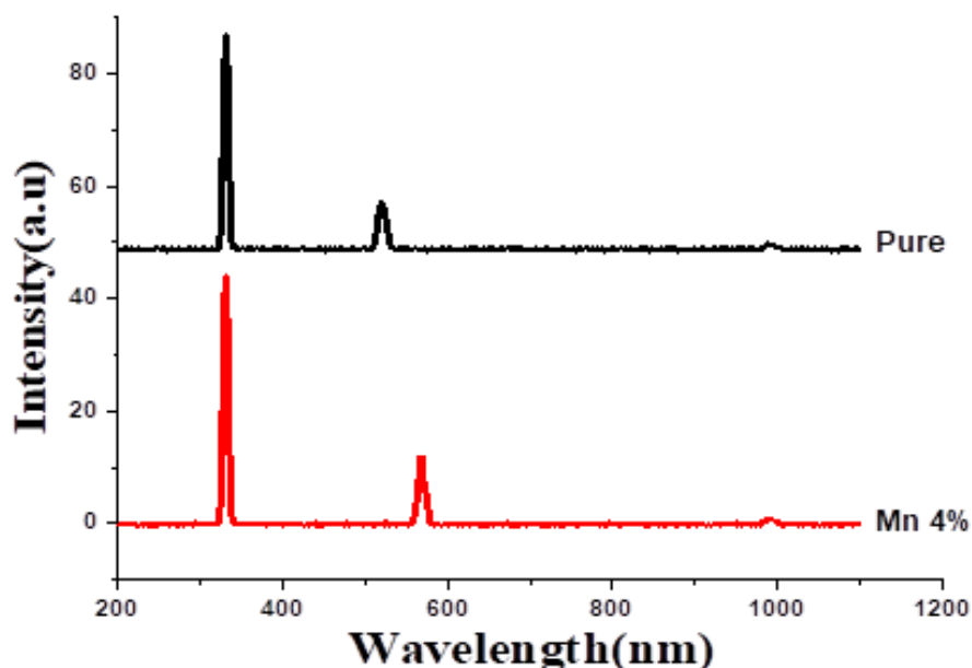
Figure 5: Photoluminescence spectra for the Pure CdS and doped CdS by Mn 4%.
